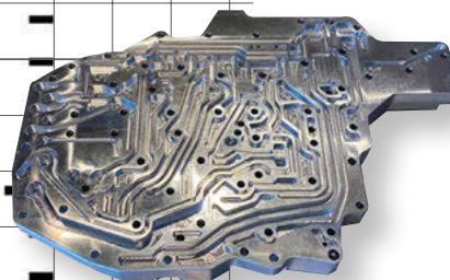
68RFE V2.0 Billet Channel Plate
